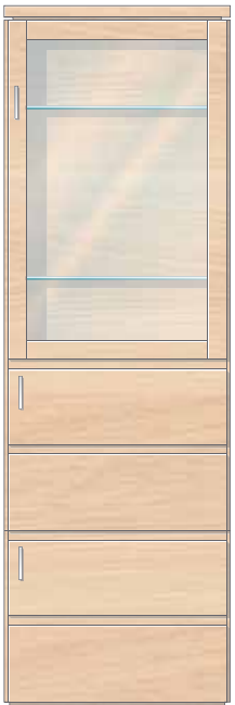
Glazed 3 Door Unit H107R All doors hinged on right (shown) H107L All doors hinged on left Internal light and two adjustable glass shelves in glazed section. H1930 x W520 x D430mm H76 x W20½ x D17 inches
