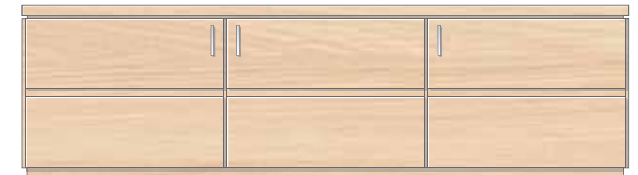
3 Door Base Unit H323 H510 x W1555 x D430mm H20 x W61¼ x D17 inches
