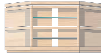
Open Corner Base Unit H402 One central fixed wooden shelf and two removable glass shelves. One removable wooden shelf in each side section. H510 x W800 x D770mm H20 x W31½ x D30¼ inches Length along wall from corner 800mm – 31½ inches
