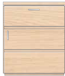
1 Door/1 Drawer Base Unit H105R Hinged on right (shown) H105L Hinged on left H750 x W520 x D430mm H29½ x W20½ x D17 inches
