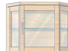
Glazed Corner Wall Unit H143R Hinged on right (shown) H143L Hinged on left Internal light. One adjustable glass shelf. H490 x W520 x D485mm H19¼ x W20½ x D19 inches Length along wall from corner 540mm – 21¼ inches
