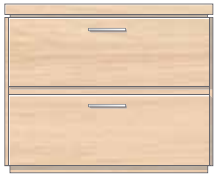
2 Drawer Base Unit H102 H510 x W520 x D430mm H20 x W20½ x D17 inches
