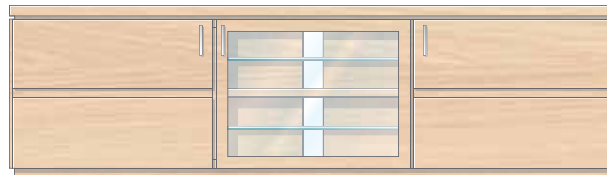
Glazed 3 Door Media Base Unit H322 One central fixed wooden shelf and two removable glass shelves in glazed section. H510 x W1555 x D430mm H20 x W61¼ x D17 inches
