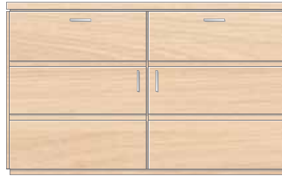
2 Drawer/2 Door Base Unit H215 H750 x W1035 x D430mm H29½ x W40¾ x D17 inches
