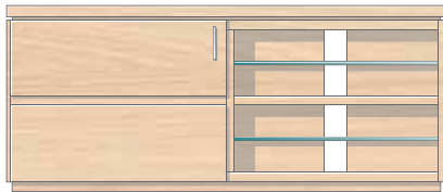
1 Door Open Media Base Unit H210 One central fixed wooden shelf and two removable glass shelves in glazed section. H510 x W1035 x D430mm H20 x W40¾ x D17 inches
